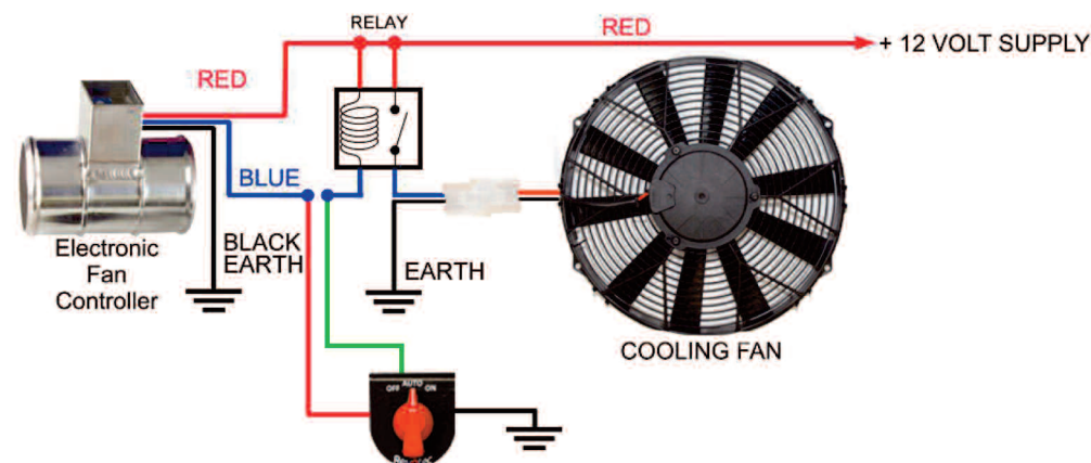
OVER RIDE SWITCH CONNECTIONS
